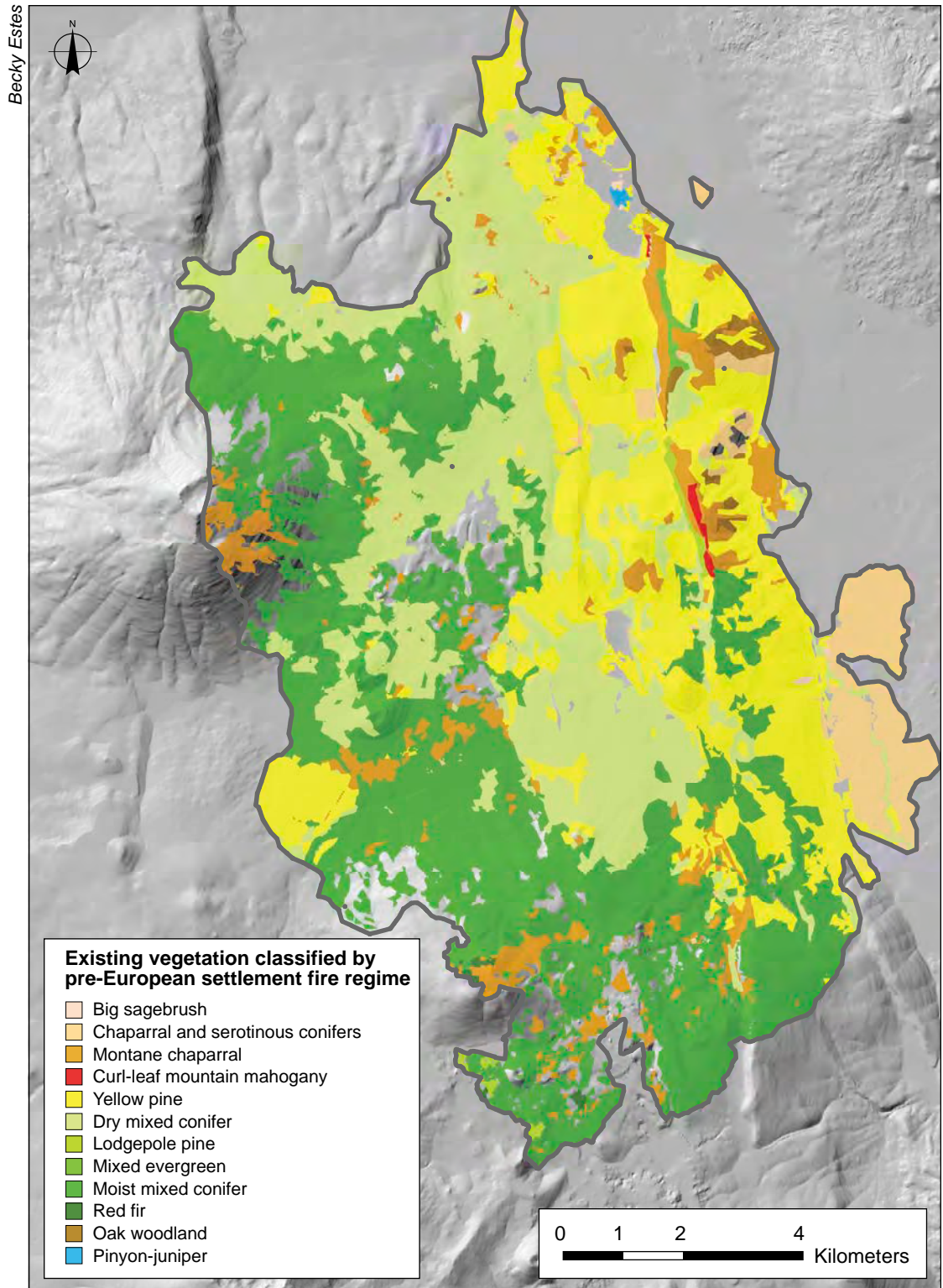
Figure 3.2—Prefire existing vegetation reclassified as pre-Euro-American settlement fire regimes within the Eiler Fire (2014) perimeter on the Lassen National Forest.
