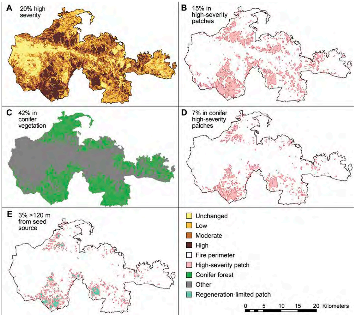
Figure A4.1—Different considerations for characterizing spatial patterns of high-severity fire for the 2015 Rough Fire. Based on the simple classification (thresholds from Miller and Thode 2007) 20 percent of the fire area is high severity (A). Using the PatchMorph tool to delineate contiguous patches of high severity, 15 percent of the area was included in patches (B). This percentage was further reduced when only conifer vegetation (C) was considered in the delineation of high-severity patches, resulting in 7 percent of the fire area (D). Considering conifer-dominated areas in high-severity patches that were >120 m from live conifers, this percentage was reduced to 3 percent (E).
