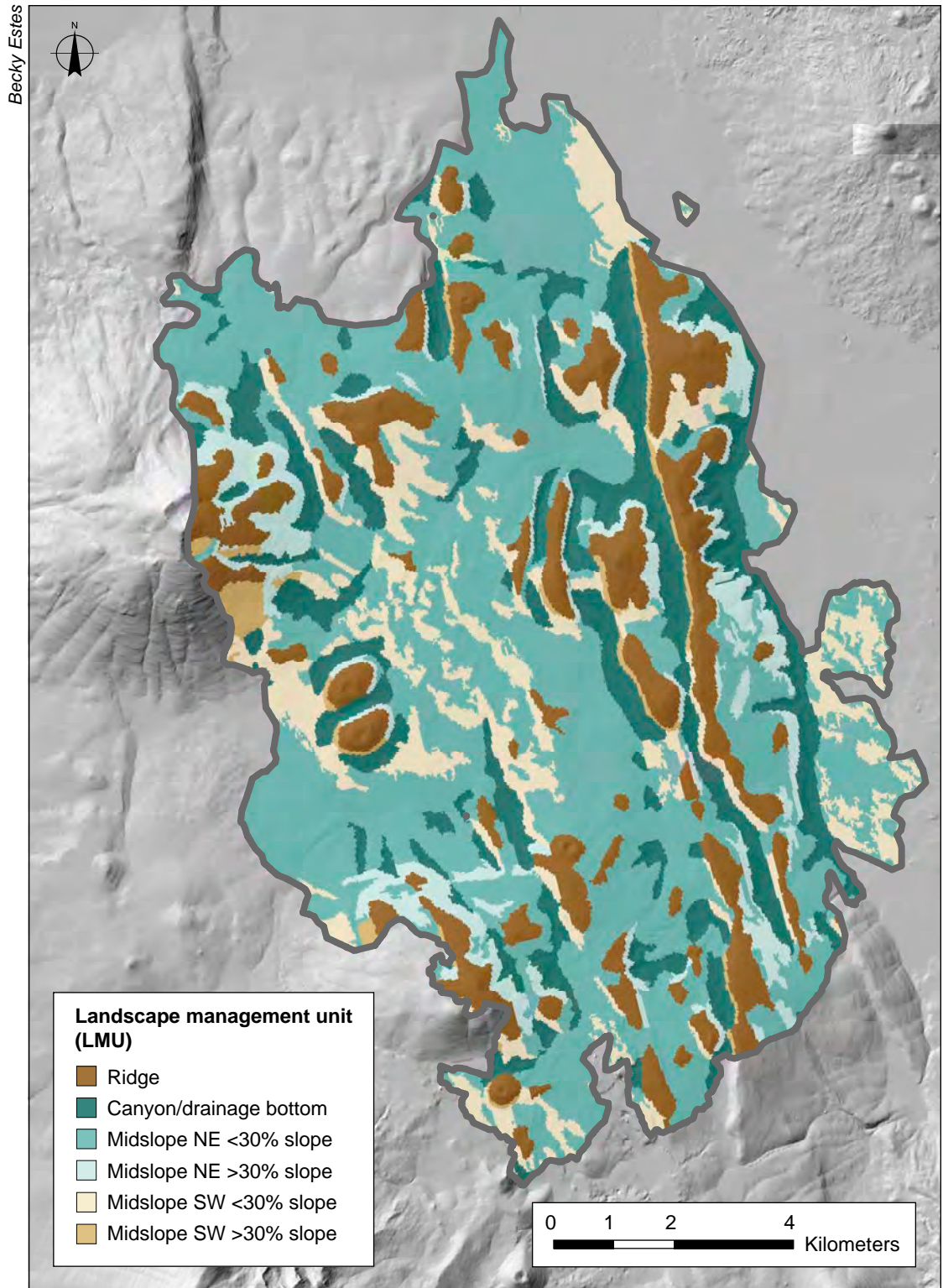
Figure 3.3—Landscape position classified by the landscape management unit tool within the Eiler Fire (2014) perimeter on the Lassen National Forest. Canyons and drainages are shown in dark blue and ridges are shown in dark brown.
